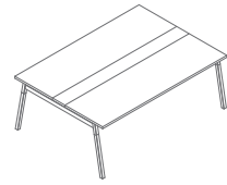
SW48 1800 / 1410 / 740 75.5 kg
