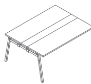
SW26L 1600 / 1210 / 740 54.5 kg
