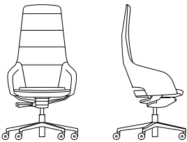
Line Soft high back W 69 – D 66 H 122÷132 / seat H 42÷52
